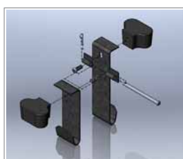
Adjustable adaptor, 2 pair
