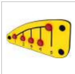
Algebra
