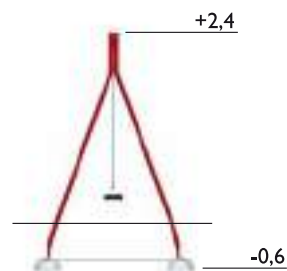
Swing set, steel Sunken foundation
