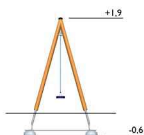
Swing set, wood Sunken foundation
